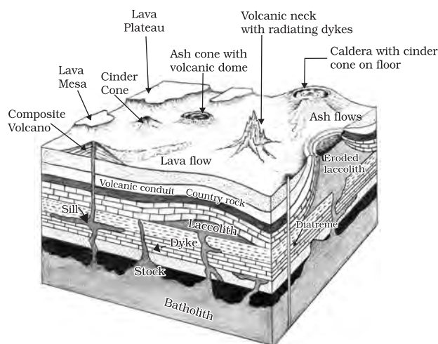
Figure 3.4 : Volcanic Landforms
